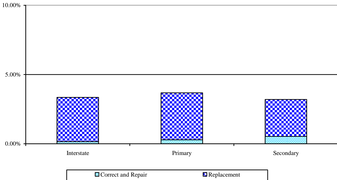
Figure A-36: Percent of guardrail terminals needing work on VDOT maintained highways - by System
